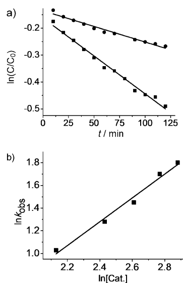
Figure 2. a) Plot of \ln(C/C_0) versus time for the cyclization of 2 ( \blacksquare ; substrate of Table 1, entry 2) and [D_2]2 ( \bullet ) catalyzed by 1 in C_6D_6 at 25 °C. For [D_2]2 : y = -0.00116x - 0.13541 , R^2 = 0.97333 ; For 2 : y = -0.00281x - 0.16261 , R^2 = 0.98849 . b) Plot of \ln k_{obs} versus \ln [Cat.] for the cyclization of 2 by 1 in C_6D_6 at 25 °C (van't Hoff plot). y = 1.04811x - 1.23556 , R^2 = 0.98007 .
